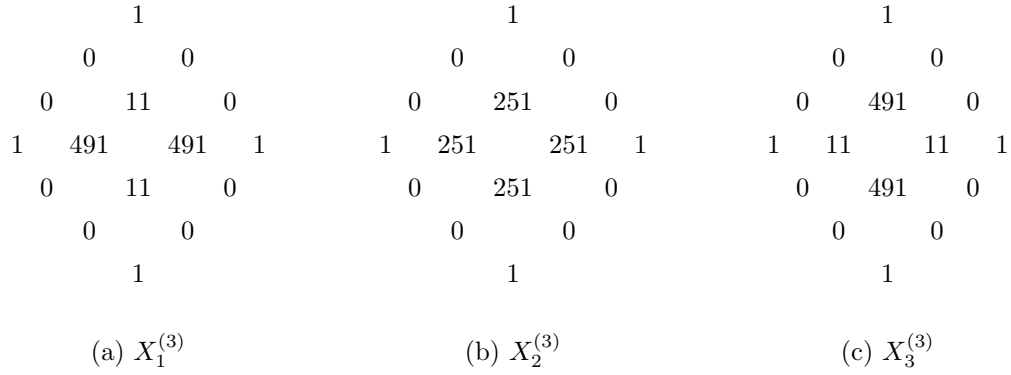
Figure 2: The orbifold Hodge diamonds of three extreme Calabi–Yau 3-folds.
