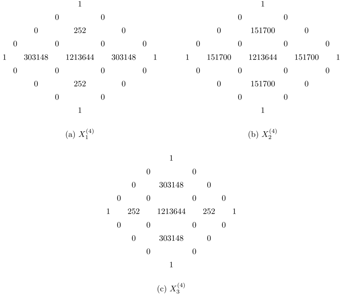
Figure 3: The orbifold Hodge diamonds of three extreme Calabi–Yau 4-folds.
