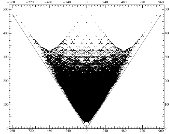
Figure 1: Hodge numbers of the Calabi–Yau 3-folds found by Kreuzer and Skarke; the x -axis is \chi = 2(h^{1,1} - h^{2,1}) , and the y -axis is h^{1,1} + h^{2,1} .
