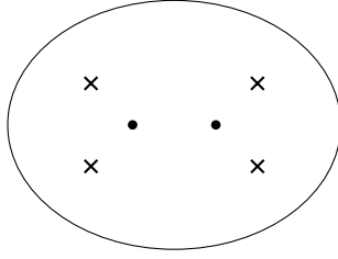
FIGURE 4. In the fourth test family, we blow up the plane at four fixed points (crosses) and two variable points (solid dots).
