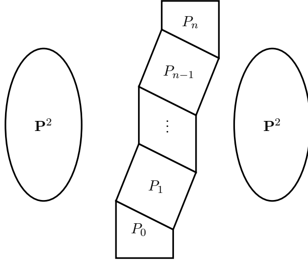
FIGURE 6. A family of surfaces with an accordion-like central fiber arises while resolving a linear rational map \mathbf{P}_R^2 \dashrightarrow \mathbf{P}_R^2 .
