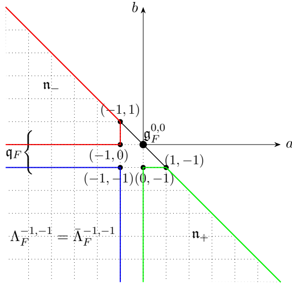
FIGURE 1. Decomposition of \mathfrak{g}_{\mathbb{C}}
